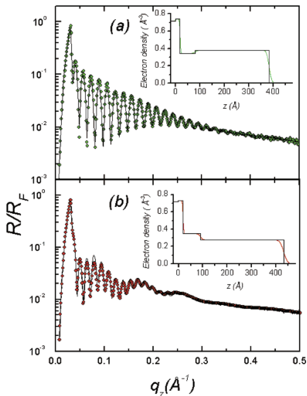
Figure 5. Measured X-ray reflectivity (circles) of the P(S-b-MMA) thin films (a) before swelling and (b) after swelling. The solid line in the figure is a fit to the experimental data, calculated using the electron density b/V profile shown in the inset.
